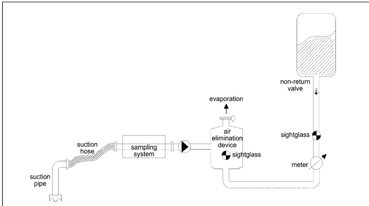
Figure 1b: Principal instrumentation of a milk measuring system, with suction by a pump
