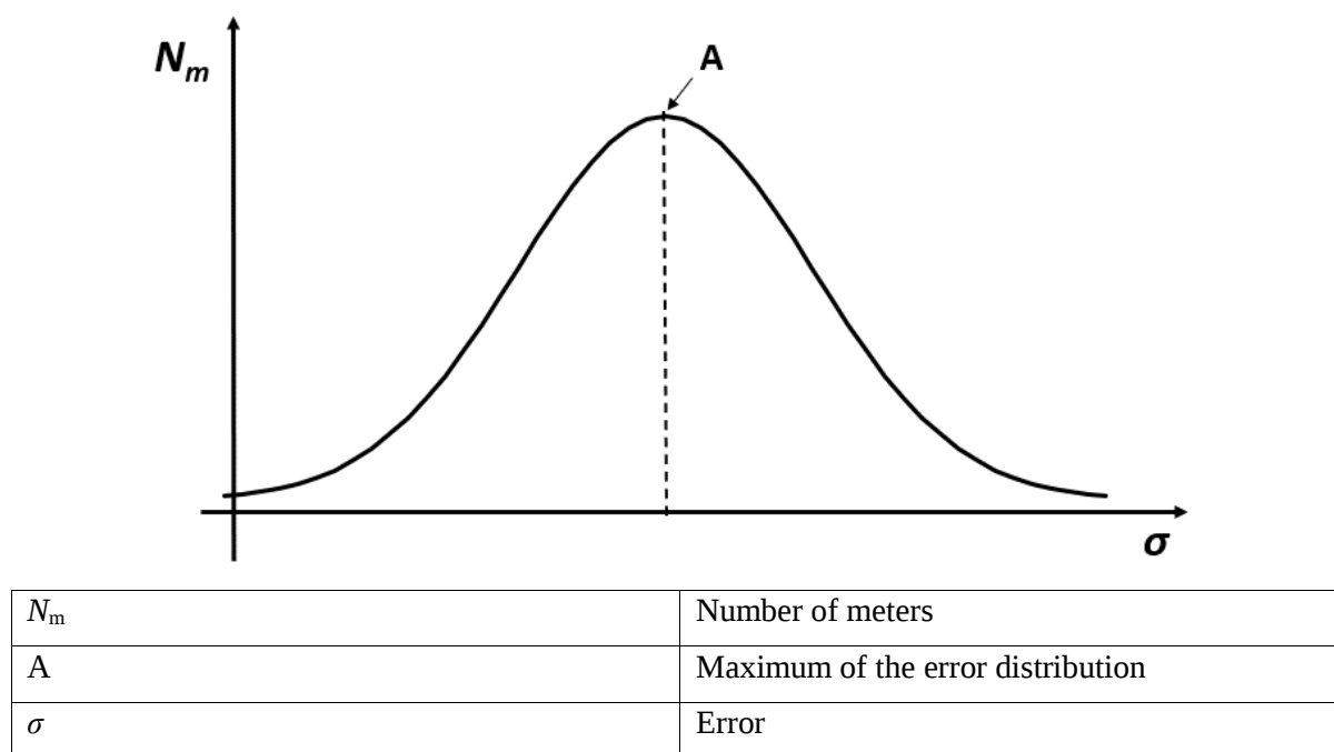
Figure 4 — Error distribution
