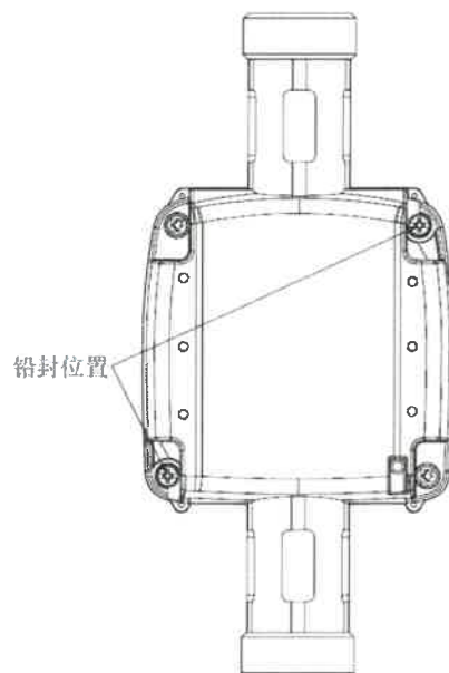
Fig. 3: Sealing of water meters type MA408
