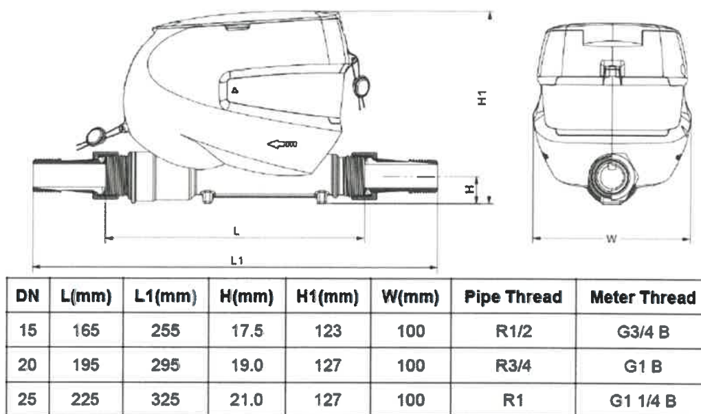
Fig. 2a: Dimensions of water meters LXCZ
