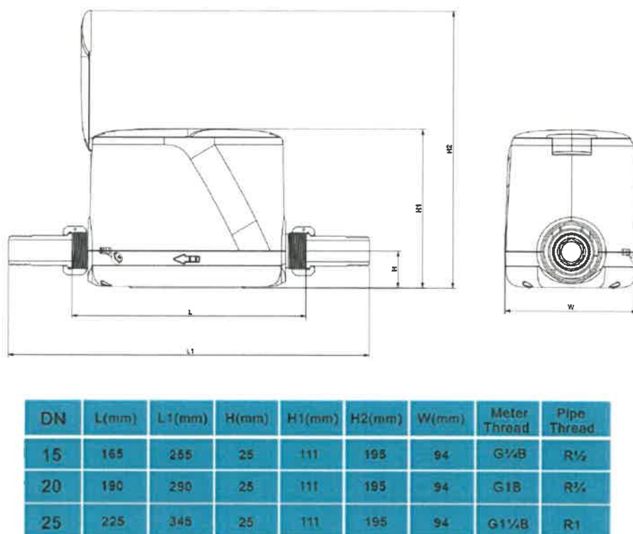
Fig. 2b: Dimensions of water meters LXCZ with pressure sensor
