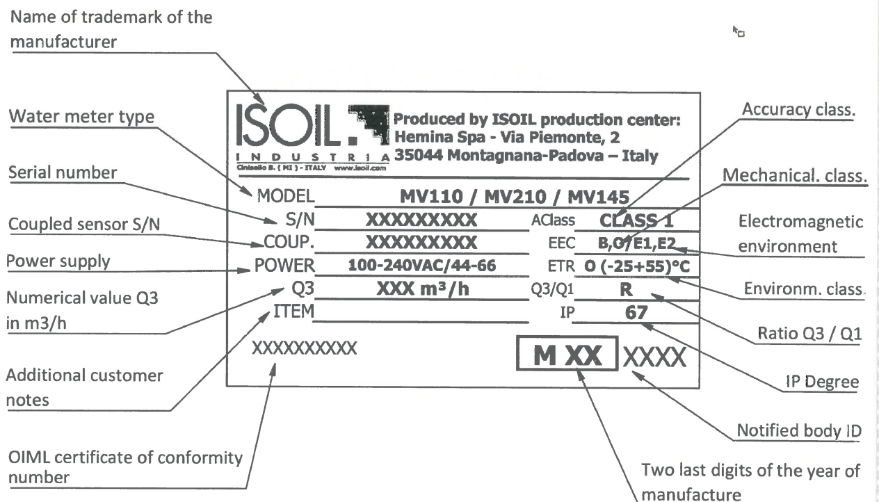
Figure 5: The labels of water meter MS2500 / MV110, MS2500 / MV210 HV or MS2500 / MV145
