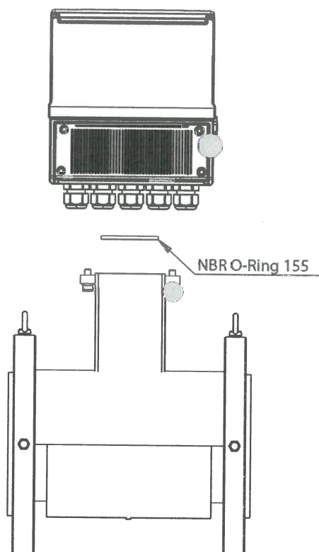
Figure 3: Sealing of The compact water meter MS2500 / MV110, MS2500/ MV210 and MS2500 / MV145
