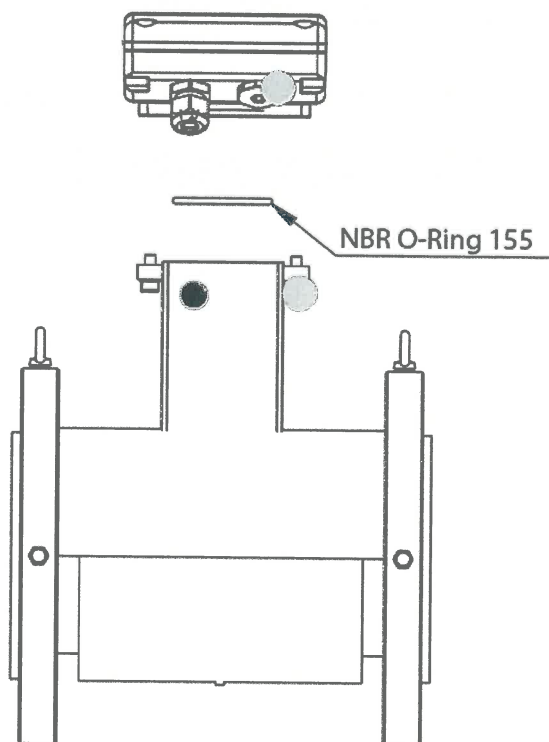
Figure 4: The sealing of the the separate water meter MS2500/ MV110, MS2500/ MV210 and MS2500 / MV145.
