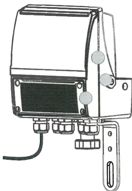
Figure 1: Sealing of the converter MV110, MV210 and MV145 of water meter compact or separate version
